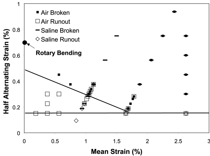
Fig. 3: Alternating strain vs. mean strain data for the 4-point bending test conducted in air and Saline solution. Rotary bending limit for zero-mean strain from Fig. 2 is added for reference.
