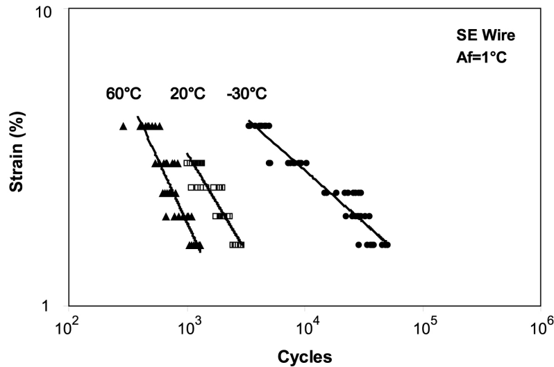
Fig. 2: Rotary bend data for superelastic wire (bright surface) tested at different temperatures
