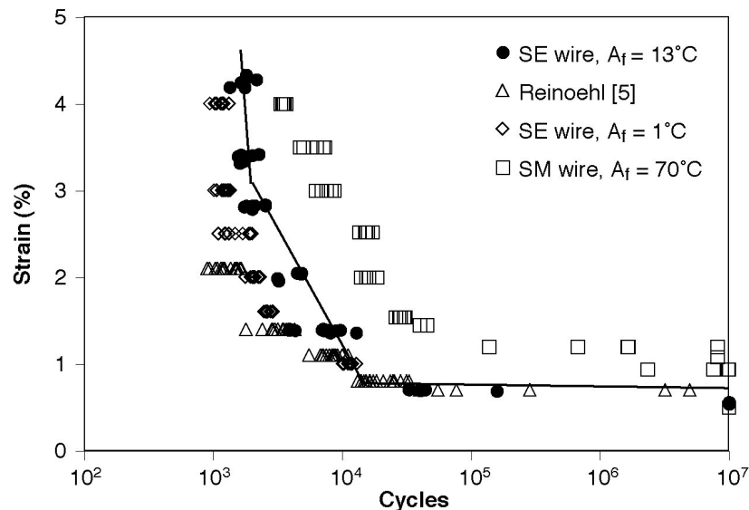
Fig. 1: S-N curves for different Nitinol wires tested at room temperature.
