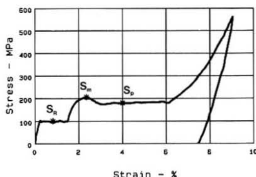
Figure 2: Strain controlled stress-strain curve conducted at -196 C.
