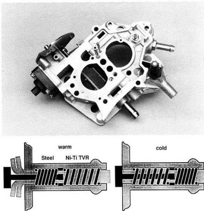
Fig. 16. Carburetor with integrated TVR ventilation valve (Solex).
