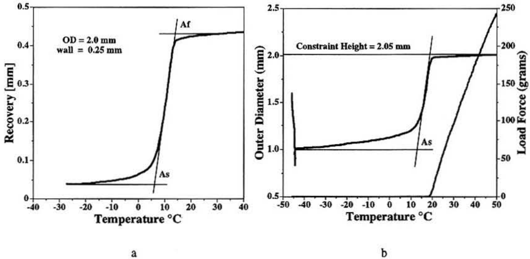
Figure 2a: Tube expansion as a function of temperature in an unconstrained recovery test. A_f is measured from this graph by the tangent method. 2b: Stent expansion and load in a constrained recovery test.
