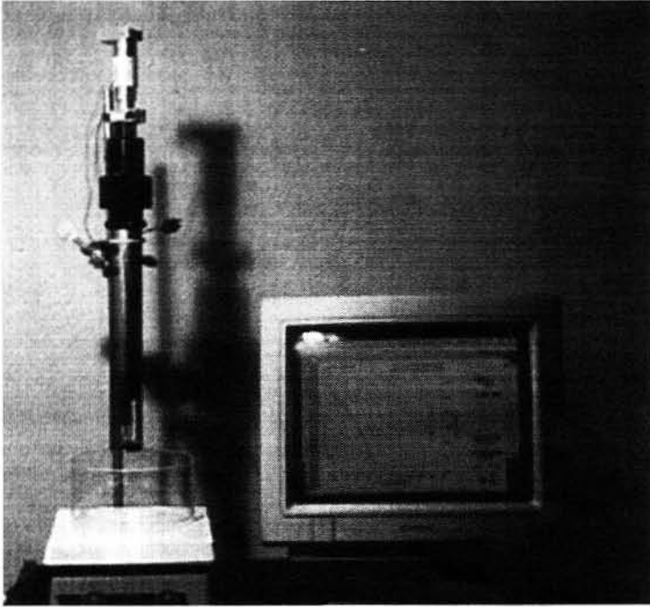
Figure 1: Apparatus for measuring austenite transition temperatures and forces exerted by stents and tubes. Samples are placed in the window near the bottom of the device.
