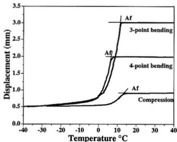
Figure 3: A_f as determined by three-point bending, four-point bending, and compression.
