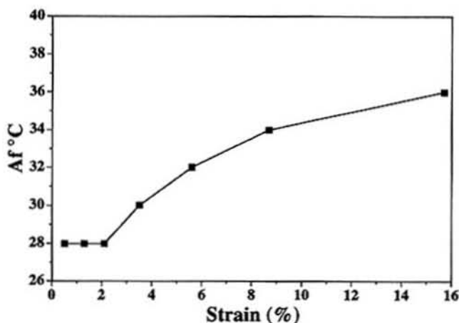
Figure 4: A_f as a function of strain. Tube dimensions: OD = 2.19 mm, wall = 0.09 mm. Transformation temperature is not a strong function of strain for strains of less than 2%.
