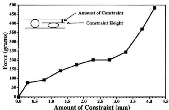
Figure 6: Stent force as a function of constraint. Note the increase in force with increase in amount of constraint. This is expected because the force measured is nearly the same as the force required to compress the stent to the given constraint level.
