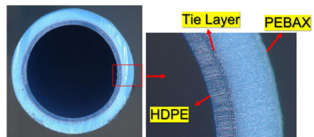
Figure 2: Optical microscopy of the cross-section of the nominal tube.
