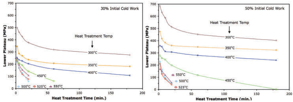
Figure 11: Trends in LP stress of 30% and 50% cold-worked Nitinol wire after heat treatment at a range of temperatures.
