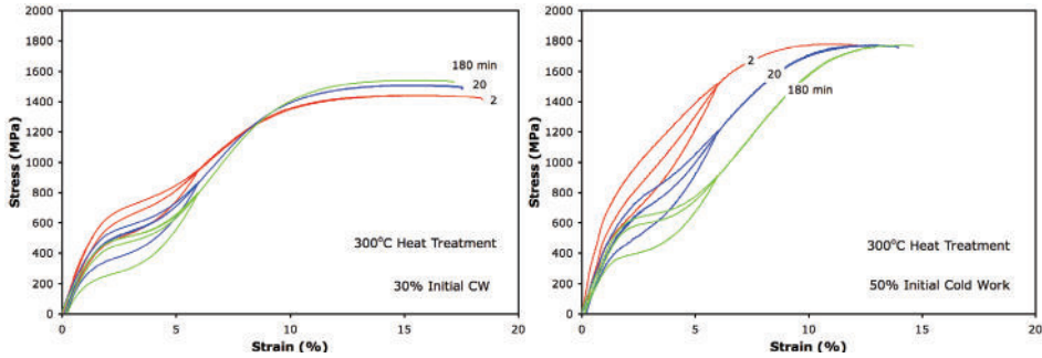
Figure 7: Tensile responses of 30% and 50% cold-worked Nitinol wires after heat treatment at 300 °C.
