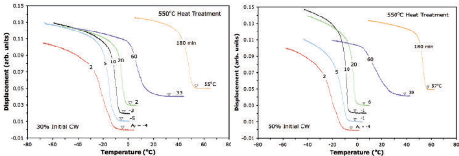
Figure 4: Representative BFR curves for 30% and 50% cold-worked Nitinol wires after heat-treatment at 550°C.
