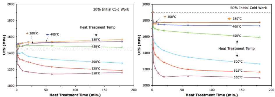
Figure 8: Trends in UTS of 30% and 50% cold-worked Nitinol wires during heat treatment at a range of temperatures.
