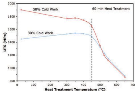
Figure 9: UTS of 30% and 50% cold-worked Nitinol wires after 60-minute heat treatments at a range of temperatures.
