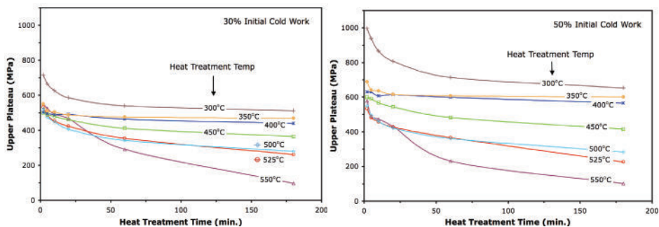
Figure 10: Trends in UP stress of 30% and 50% cold-worked Nitinol wires after heat treatment at a range of temperatures.
