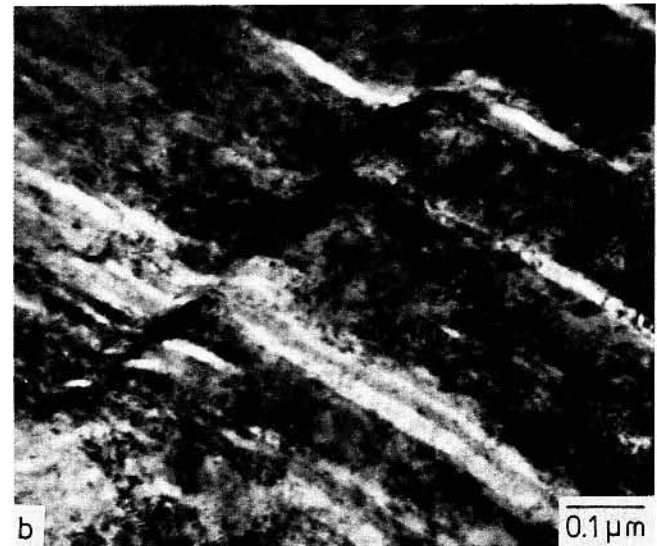
Fig. 11—Plastic deformation close to fracture in an (\alpha + \beta) ST plus \alpha -aged microstructure, 30 pct \alpha_p , \sigma_{0.2} = 1238 MPa, \epsilon_F = 0.17 , TEM.
