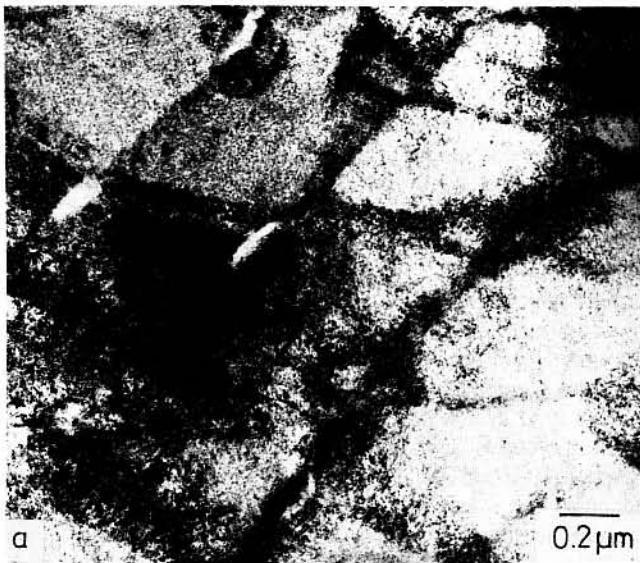
Fig. 14—Microscopic deformation in an ( \alpha + \beta ) ST plus \omega -aged microstructure, 30 pct \alpha_p , recrystallized, \epsilon_F = 0.31 , TEM. (a) Intersecting slip bands, (b) offsets at grain boundaries caused by intense slip bands.
