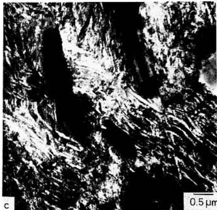
Fig. 10—Plastic deformation close to fracture in an (\alpha + \beta) ST plus \alpha -aged microstructure, 10 pct \alpha_p , \sigma_{0.2} = 1202 MPa, \epsilon_F = 0.63 , TEM.
