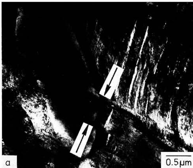
Fig. 11—Plastic deformation close to fracture in an (\alpha + \beta) ST plus \alpha -aged microstructure, 30 pct \alpha_p , \sigma_{0.2} = 1238 MPa, \epsilon_F = 0.17 , TEM.
