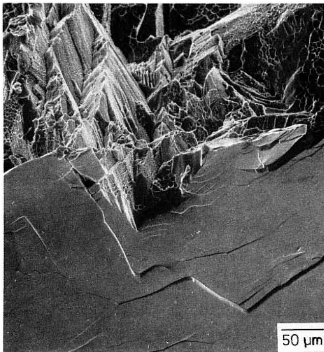
Fig. 8—Plastic deformation and fracture in a \beta -ST plus \alpha -aged microstructure, no GB \alpha , 850 °C, 2 h, WQ, 320 °C, 5 h, \sigma_{0.2} = 1588 MPa (230 ksi), \epsilon_F = 0, intersection of gage length surface and fracture surface, SEM.
