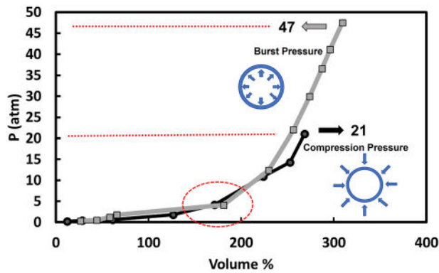
Figure 9: Burst/crush test results in a ramp method for nominal tube.
