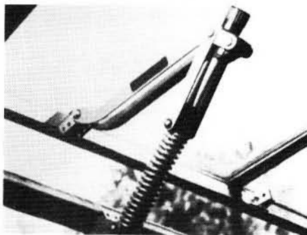
Figure 16. The first thermal actuator used a large Cu-Zn-Al spring to open and close greenhouse windows, serving both as a temperature detection device and actuator.
