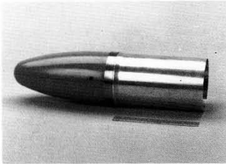
Figure 6: Large diameter, thin-walled Ni-Ti bands are used to join segments of missiles. (Raychem Corp.)
