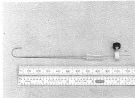
Figure 24. A superelastic Ni-Ti-V wire shaped into a hook is passed through a cannula a hooks around breast tumors to help surgeons accurately locate and remove the tumor. (Mitek Inc.)
