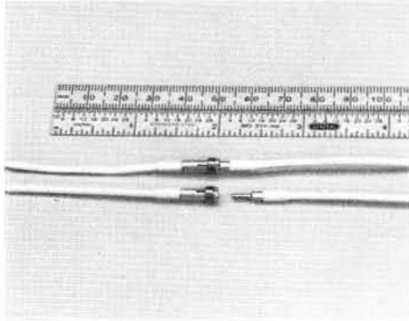
Figure 8. The first shape memory connector was the Cryocon ® : a single pin socket released by a cold freon spray. (Raychem)
