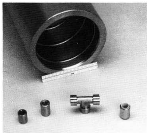
Figure 4. Shape memory couplings of various designs are used in the marine and commercial industries. From left to right are the monolithic, driver-liner, ring-body, and Permacouple designs. The largest coupling (above) is over 15 cm in diameter. (Raychem Corp.)
