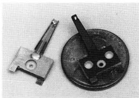
Figure 13. A prototype of a disk drive head lifter used a short piece of Ni-Ti-Cu wire to gently lift magnetic heads during shut downs. (Raychem Corp.)
