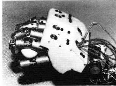
Figure 15: A robotic hand uses Ni-Ti both to provide actuation and tactile feedback. (The Furukawa Electric Co.)
