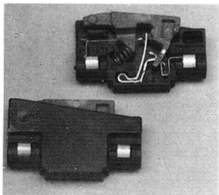
Figure 21. There have been many efforts use shape memory in circuit breakers such as the one shown above. This particular one opens a circuit when the current passing through a Ni-Ti-Cu wire exceeds a critical level. (Raychem Corp.)
