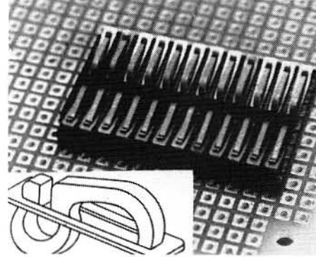
Figure 9. A Dual In-line Package socket uses shape memory to provide individual pin contacts with zero insertion forces. (Raychem Corp.)
