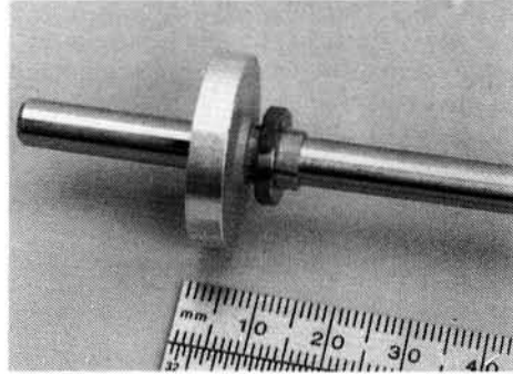
Figure 7: Small Ni-Ti ring is used to locate and fix the position of a bearing on a shaft. (Raychem Corp.)
