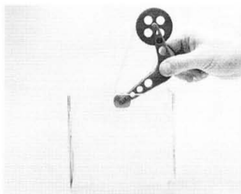
Figure 22. The Thermobile® uses the change in modulus that occurs in a loop of Ni-Ti-Co wire as it undergoes the R-phase transformation to demonstrate the concept of thermal-to-mechanical energy conversion. (Innovative Technologies)
