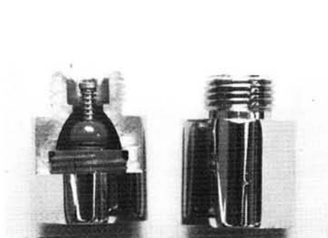
Figure 20. An anti-scald device uses a Cu-Zn-Al spring to interrupt water flow and prevent accidental scalding. (Memry Inc.)
