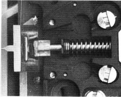
Figure 14: The SMART Clamp is one of the few electrical actuators now in production. It uses four Ni-Ti wires to control the pressure of a blade (left) on an IV tube. (Betaphase, Inc.)
