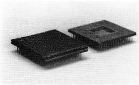
Figure 10: A Pin-Grid Array Package uses a Ni-Ti guillotine mechanism to provide exceptionally high performance with easy installation. (Raychem Corp.)
