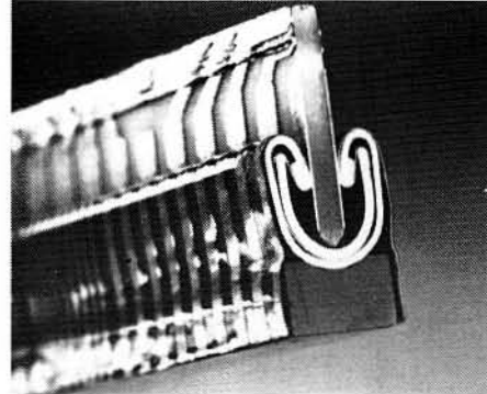
Figure 11: The new Betaflex ® connector uses the electrical heating of a Ni-Ti sheet to release a flexible polyimide ribbon imprinted with copper conductors. (Betaphase, Inc.)
