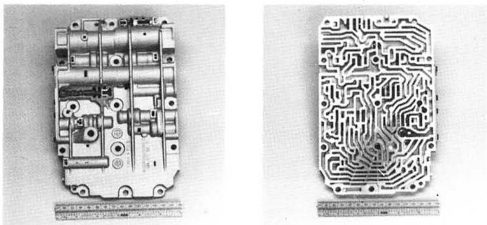
Figure 18. Three springs are used in the valve covers for automatic transmissions to control the shifting depending upon engine temperature. Shown on the left is the outside of the valve cover with two areas milled down to reveal the location of the memory springs. Shown on the right is the bottom of the cover and the fluid logic system; the memory springs control gates between various fluid passages. (Raychem Corp.)
