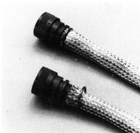
Figure 5. The most successful shape memory fastener is a welded Ni-Ti-Nb ring used to fasten a shielding braid to the back of an electrical connector shell. (Raychem Corp.)
